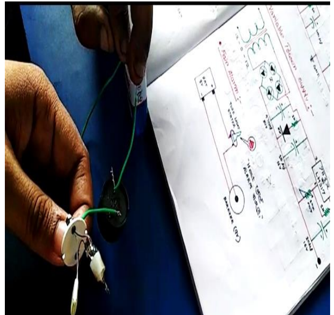
Government ITI Bauria running under PTP (DEPARTMENT :- ELECTRONICS MECHANIC) (PROJECT NAME:-FIRE ALARM)
